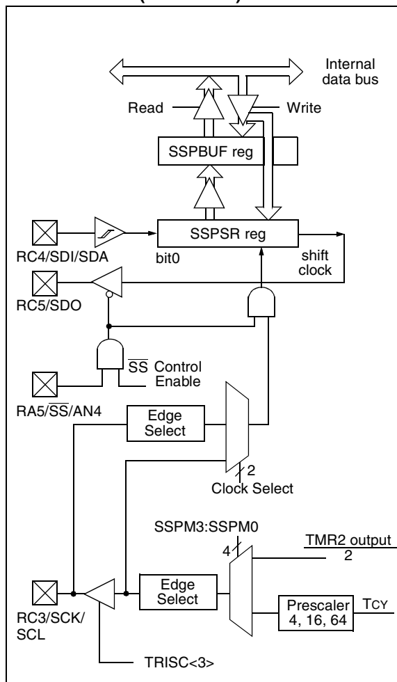
FIGURE 8-3: SSP BLOCK DIAGRAM (SPI MODE)
