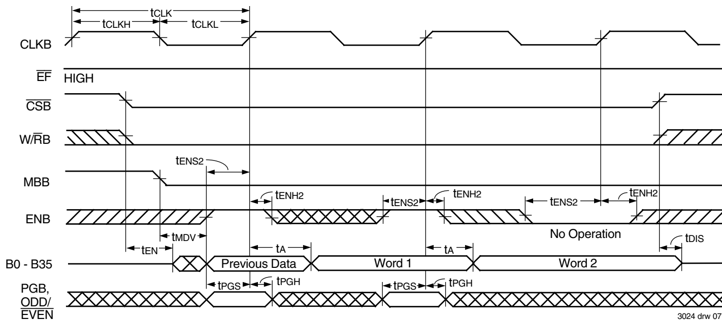
Figure 4. FIFO Read Cycle Timing
