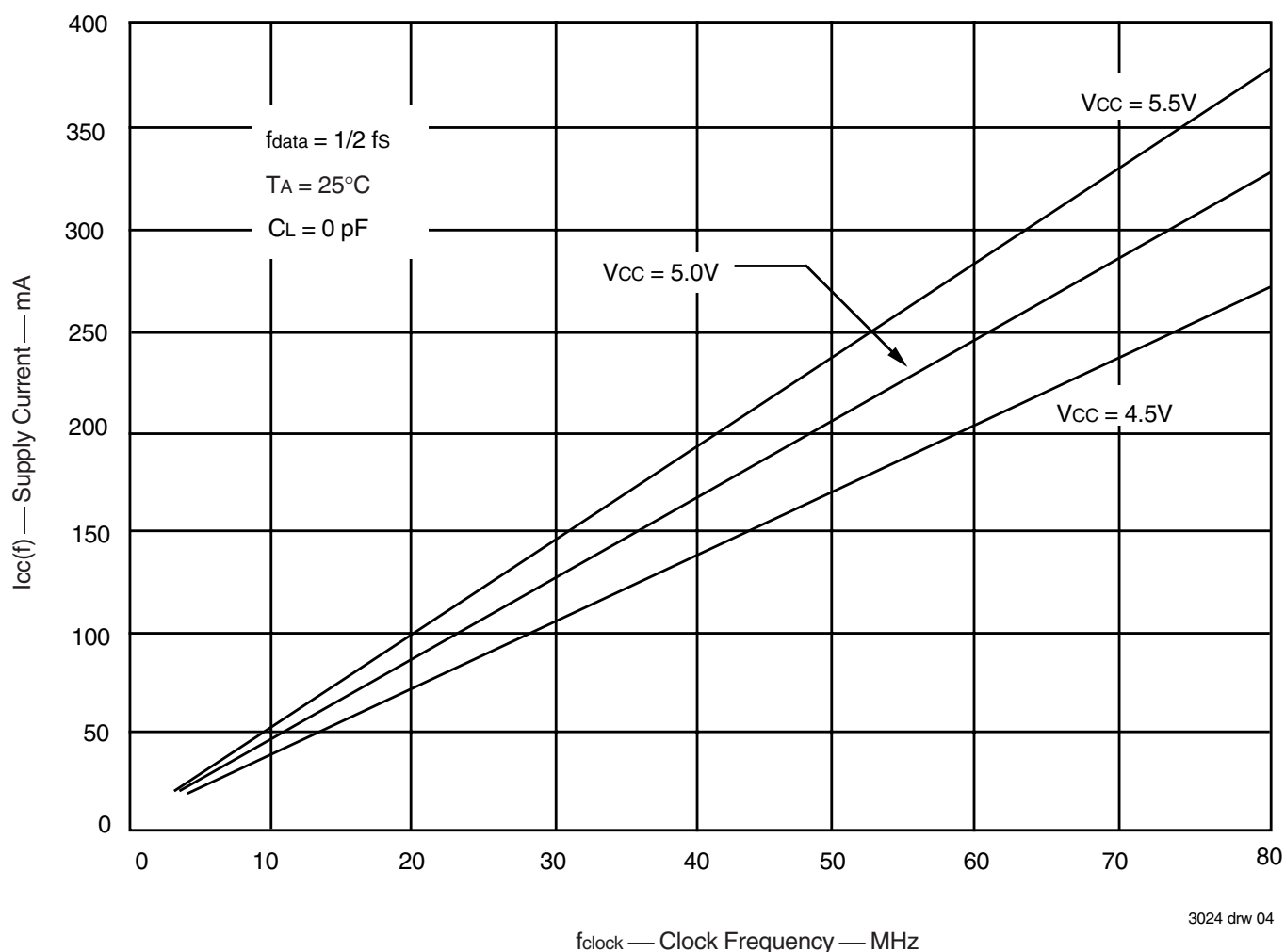
Figure 1. Typical Characteristics: Supply Current vs Clock Frequency
