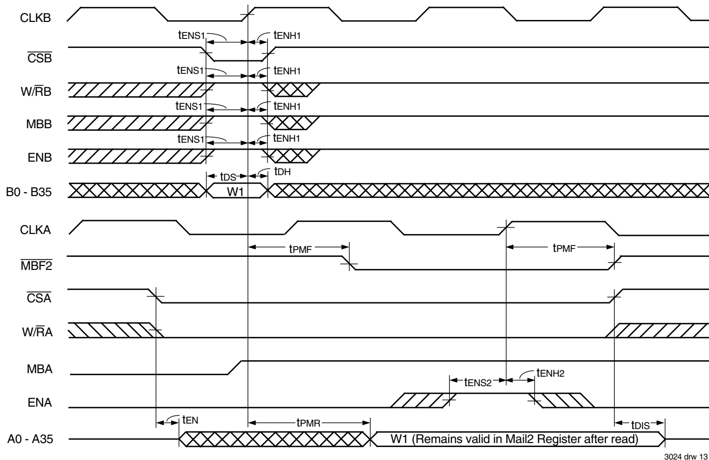
Figure 10. Timing for Mail2 Register and \overline{MBF2} Flag
