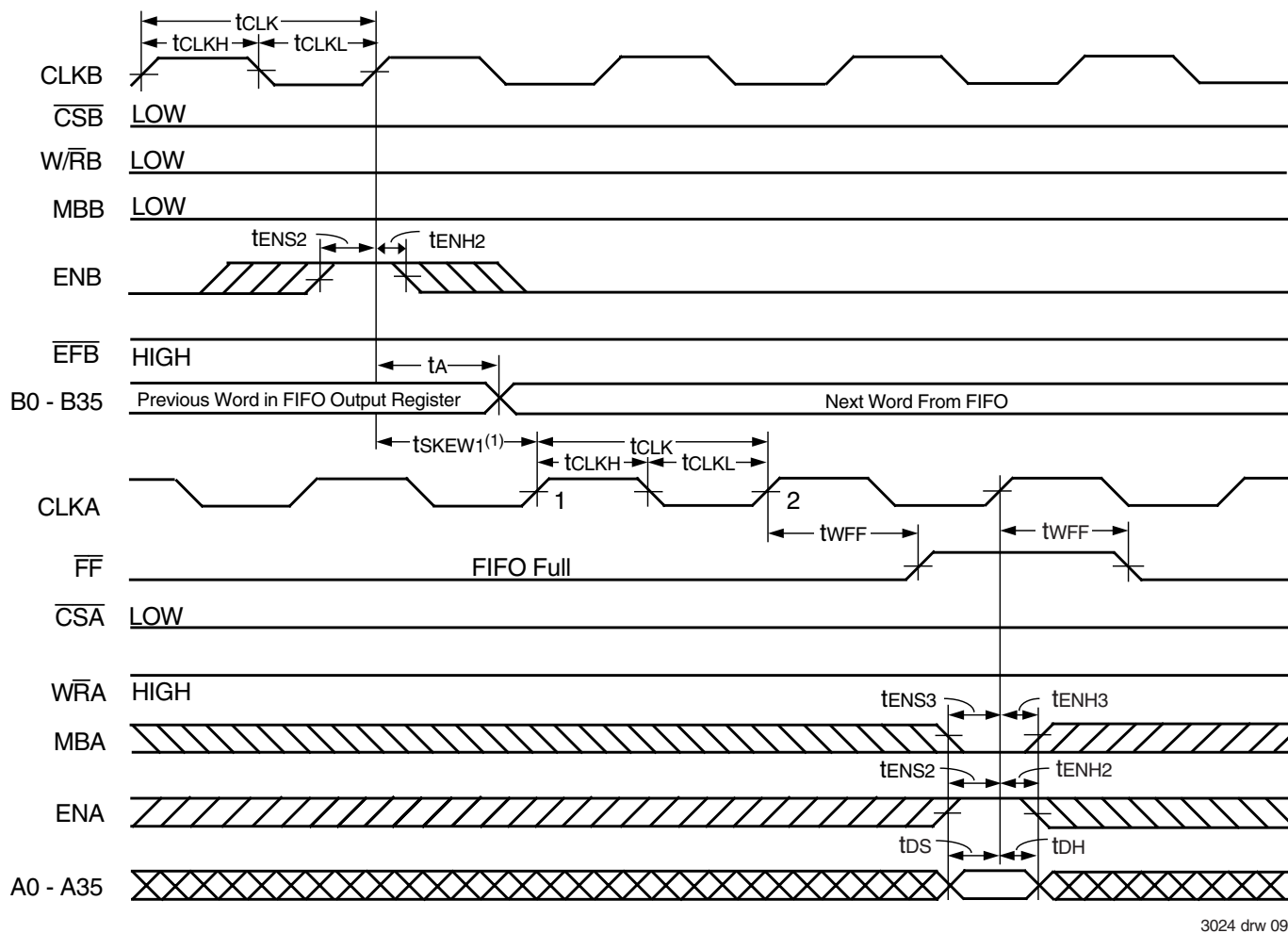
Figure 6. \overline{FF} Flag Timing and First Available Write when the FIFO is Full
