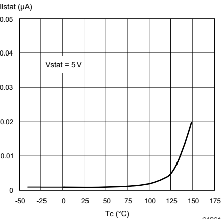
Figure 19. Status leakage current
