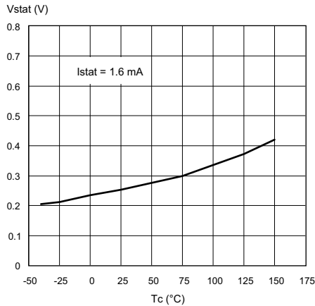
Figure 20. Status low output voltage
