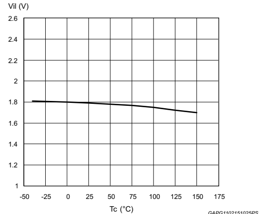
Figure 18. Input low level
