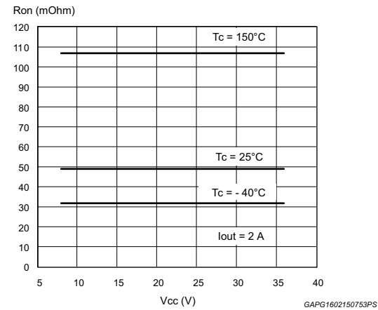
Figure 14. On-state resistance vs V_{CC}
