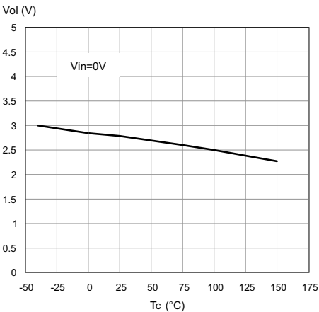
Figure 23. Open-load off-state voltage detection threshold
