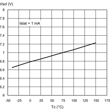
Figure 21. Status clamp voltage
