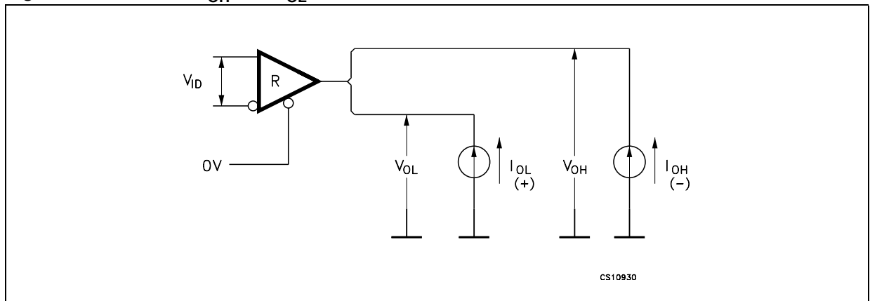
Figure 4. Receiver V_{OH} and V_{OL} test circuit
