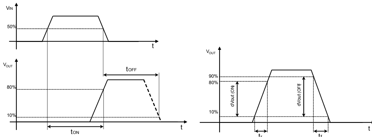
Figure 5. V_{CC} turn-ON
