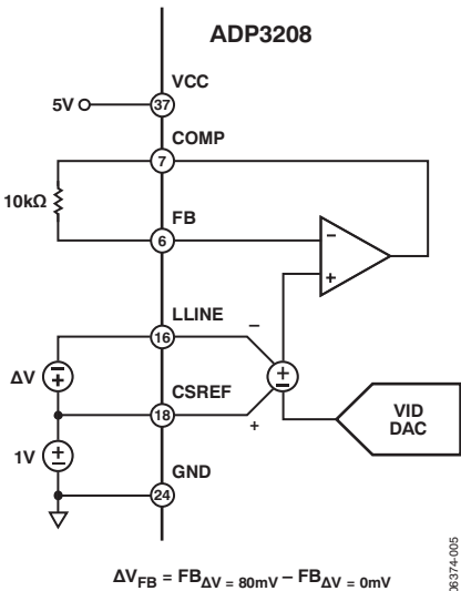
Figure 6. Positioning Accuracy
