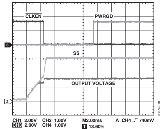
Figure 18. Start-Up Waveforms
