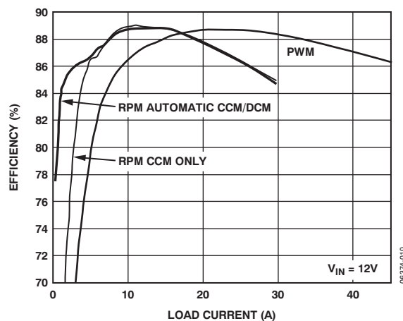
Figure 10. Efficiency vs. Load Current in All Modes
