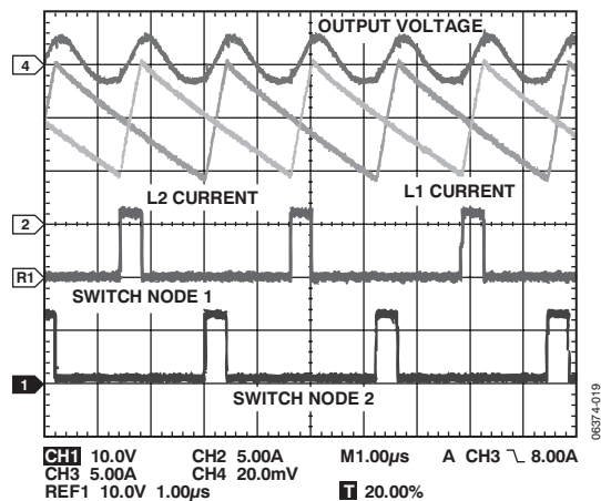
Figure 19. Dual-Phase, Interleaved PWM Waveform, 20 A Load
