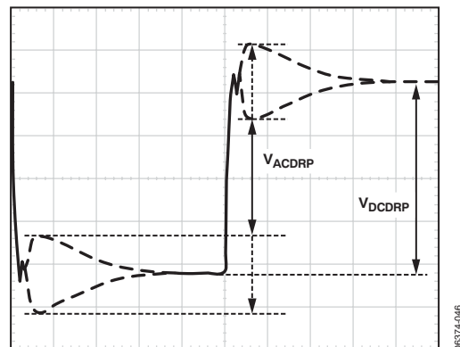
Figure 45. AC Load Line Waveform
