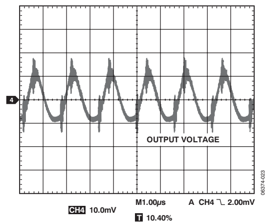
Figure 23. PWM Mode Output Ripple, 40 A Load, V_{IN} = 12\text{ V}
