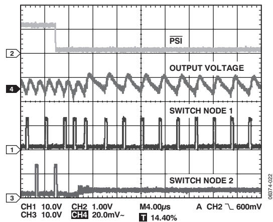
Figure 22. PSI Transition
