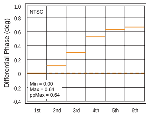
Figure 5. Differential Phase
