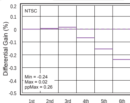
Figure 4. Differential Gain
