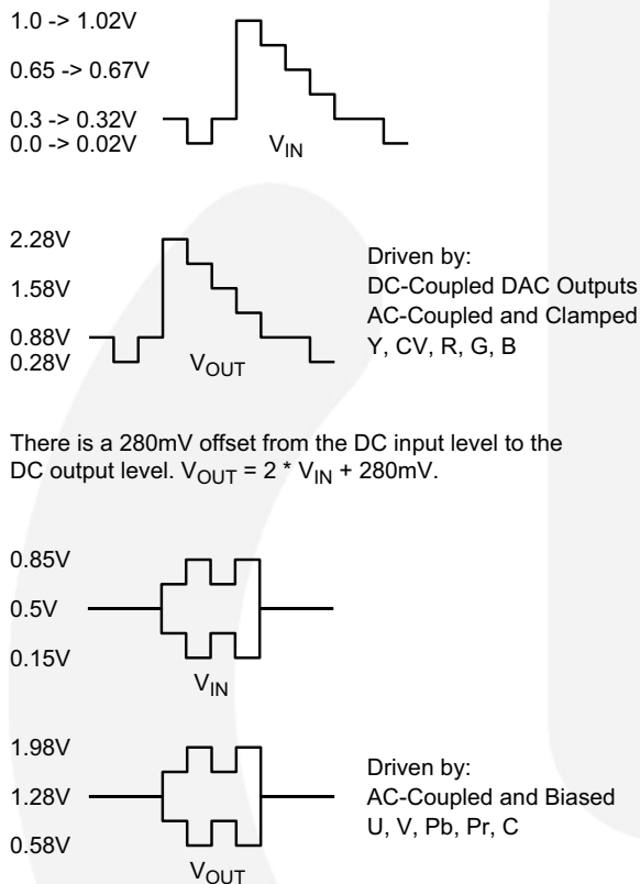
Figure 7. Typical Voltage Levels
