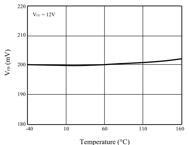
Figure 14 V_{FB} vs. Temperature
