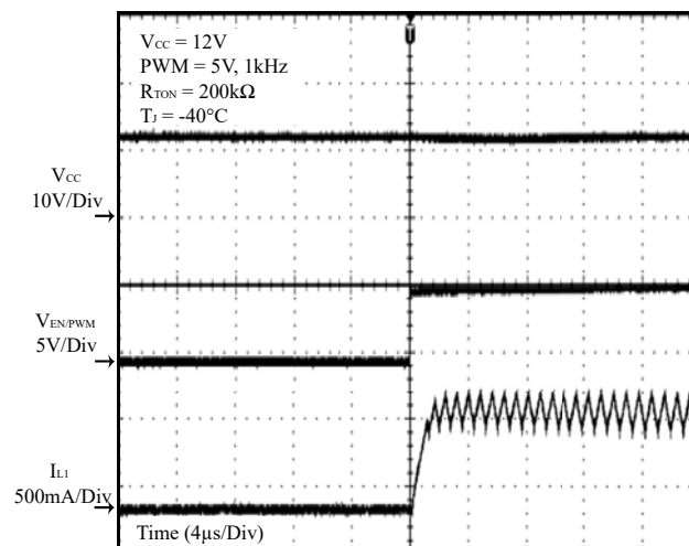
Figure 22 PWM On
