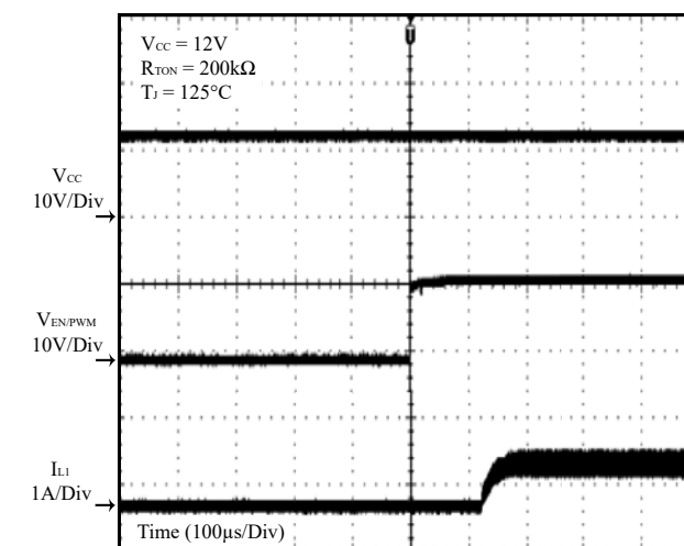
Figure 20 EN/PWM Enable Time
