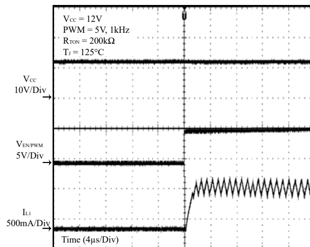
Figure 26 PWM On
