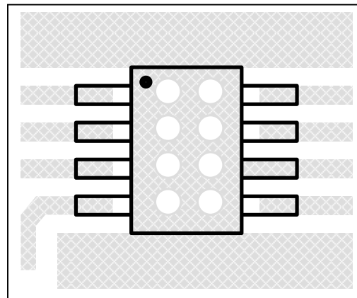
Figure 36 Board Via Layout For Thermal Dissipation
