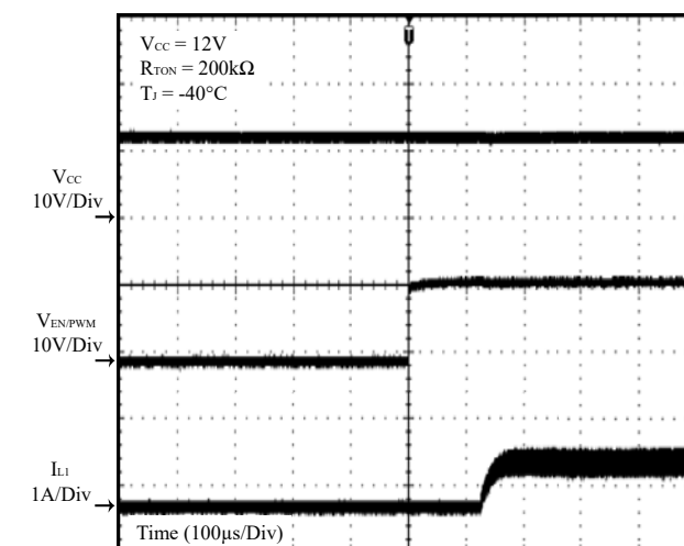
Figure 18 EN/PWM Enable Time
