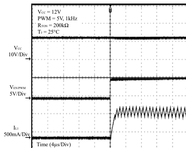
Figure 24 PWM On
