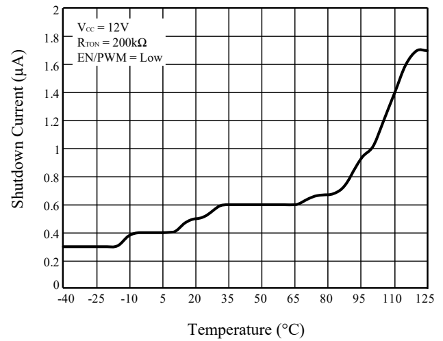
Figure 6 I_{SD} vs. Temperature
