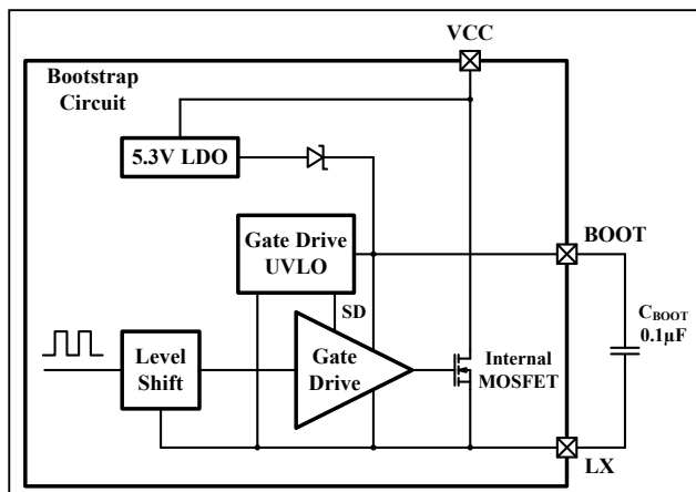
Figure 27 Bootstrap Circuit
