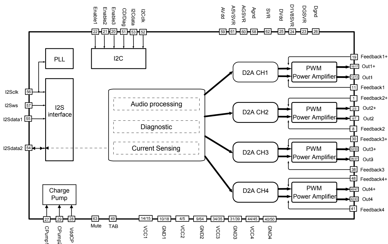
Figure 1. Block diagram
