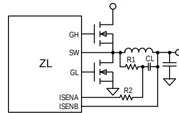
FIGURE 15. DCR Current Sensing
