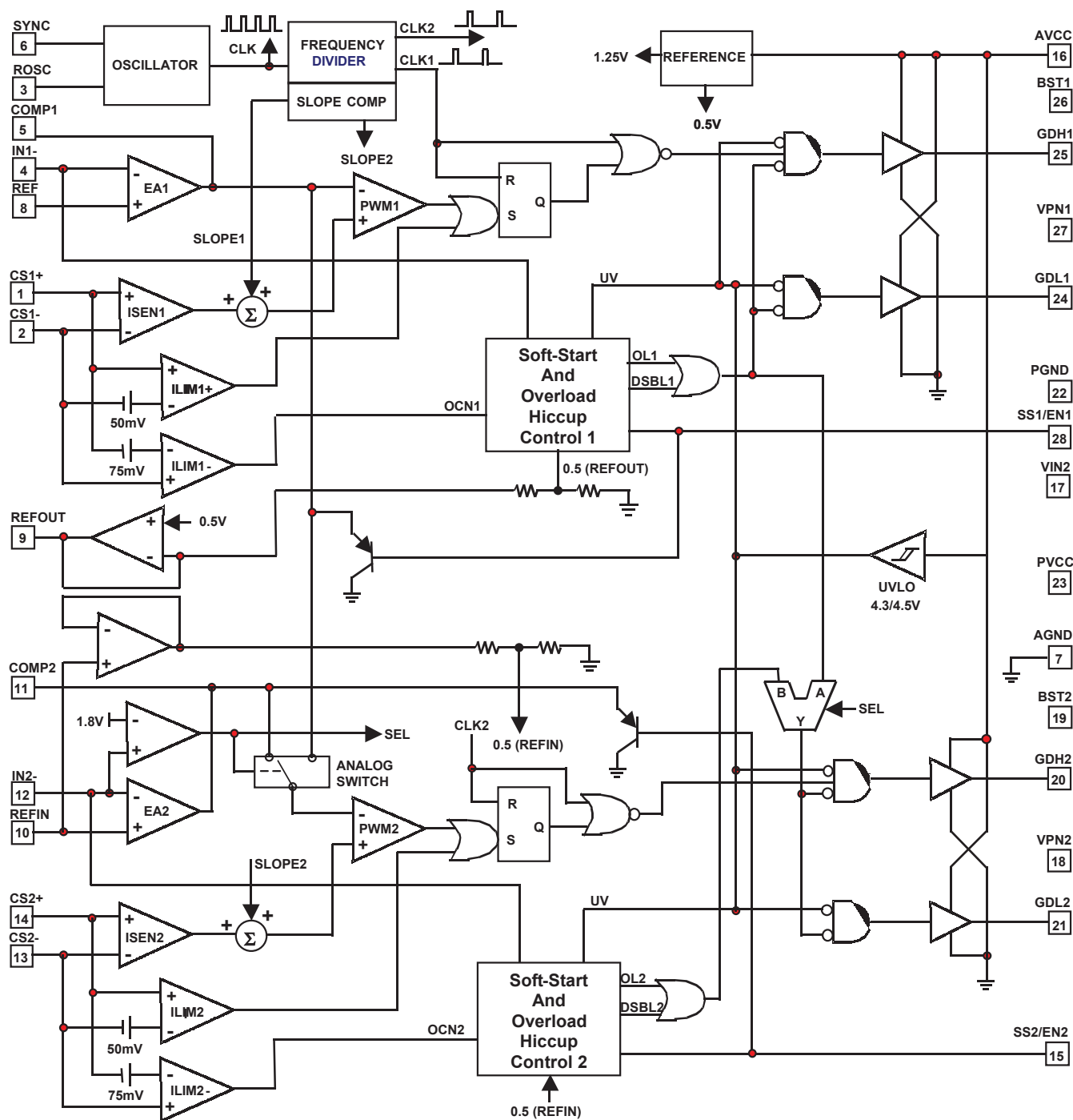
Figure 3. SC2446A Block Diagram
