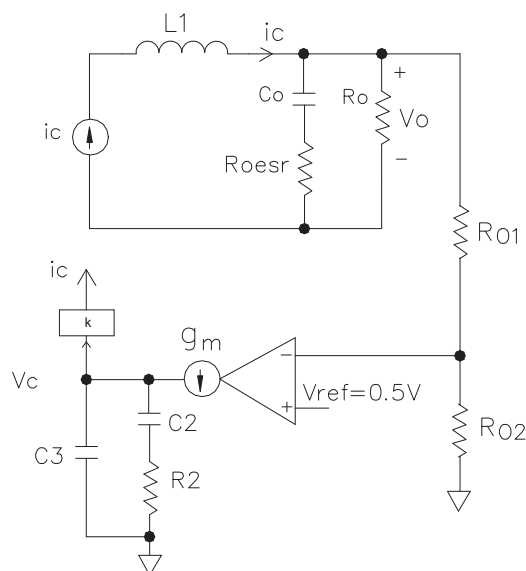
Figure 12. A simple model of synchronous buck converter with current mode control.
