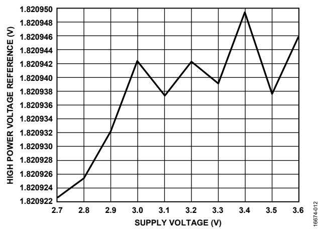
Figure 12. ADC 1.82 V Voltage Reference, DC PSRR
