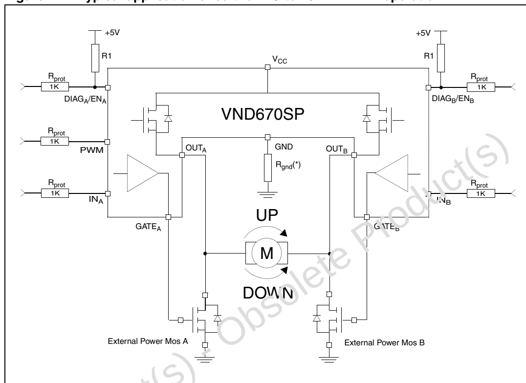
Figure 7. Typical application circuit for DC to 10 KHz PWM operation
