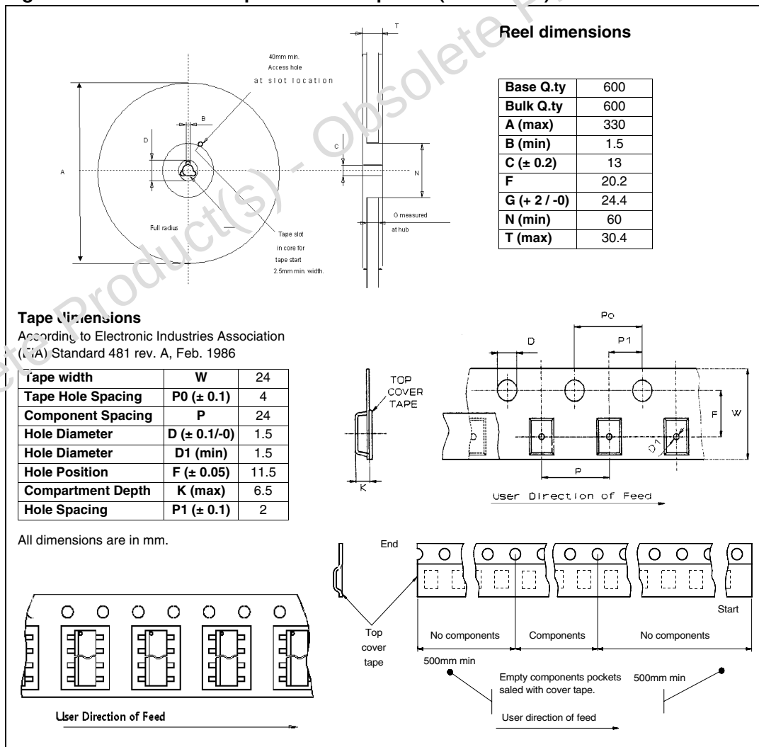
Figure 14. PowerSO-10 tape and reel shipment (suffix “R”)
