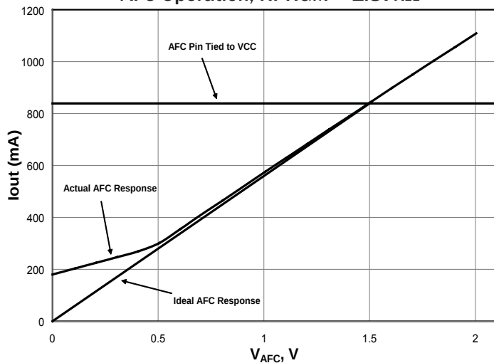
AFC Operation, RPRGM = 1.87k \Omega
