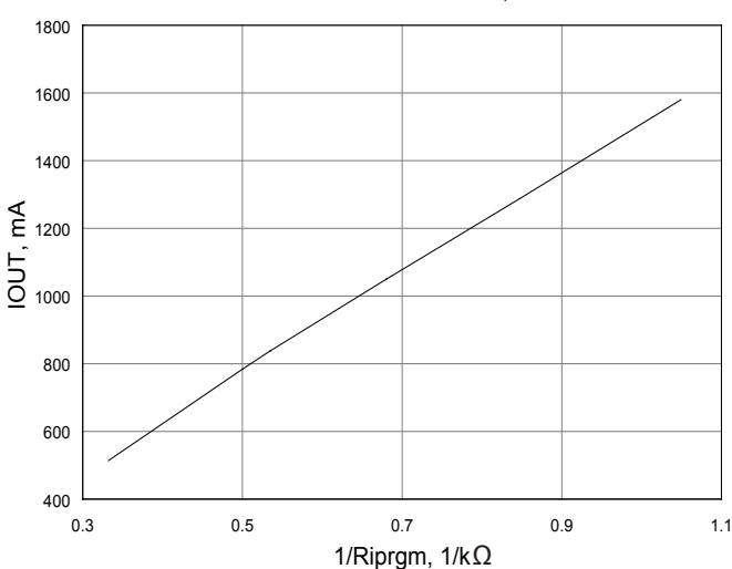
IOUT vs. IPRGM Resistance, T = +25 °C
