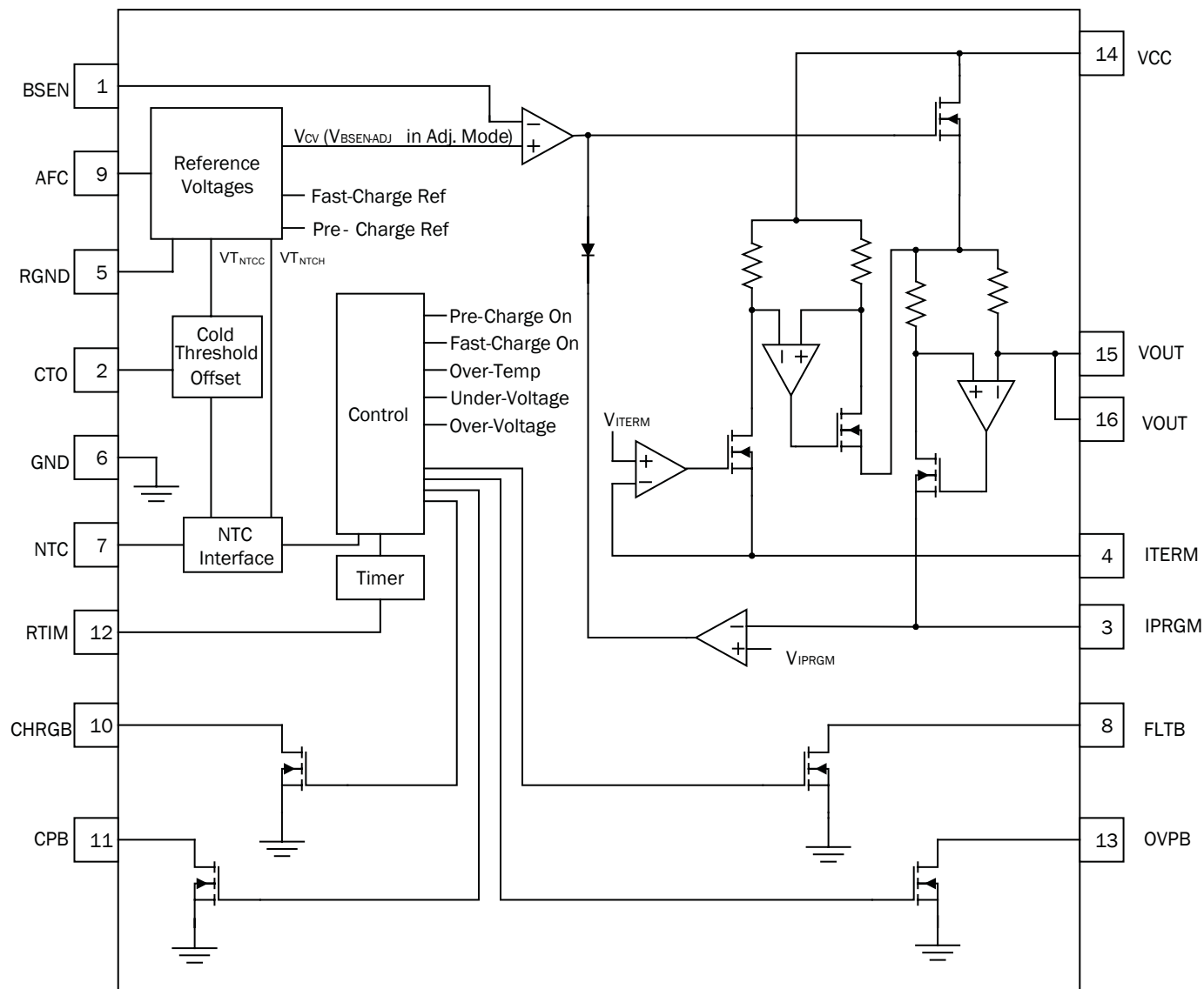
Figure 1 - SC804A Functional Block Diagram
