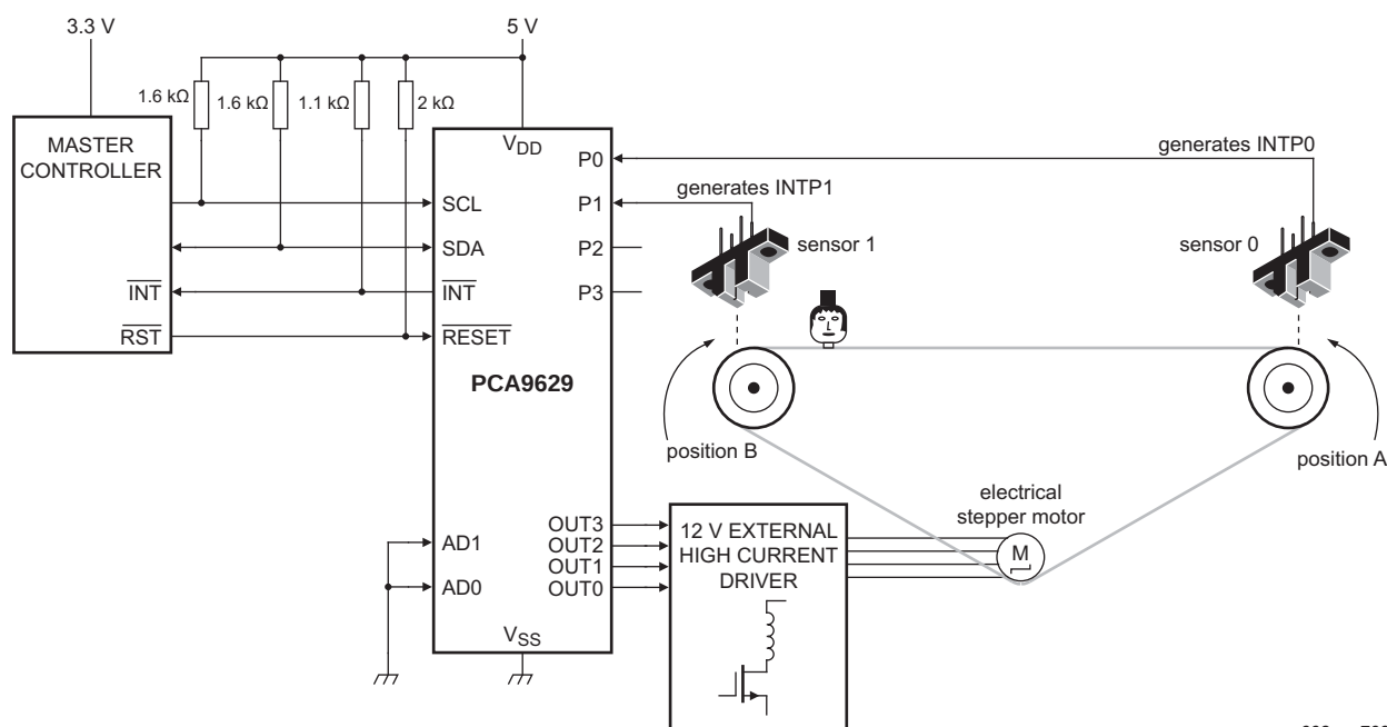
Fig 18. Typical application
