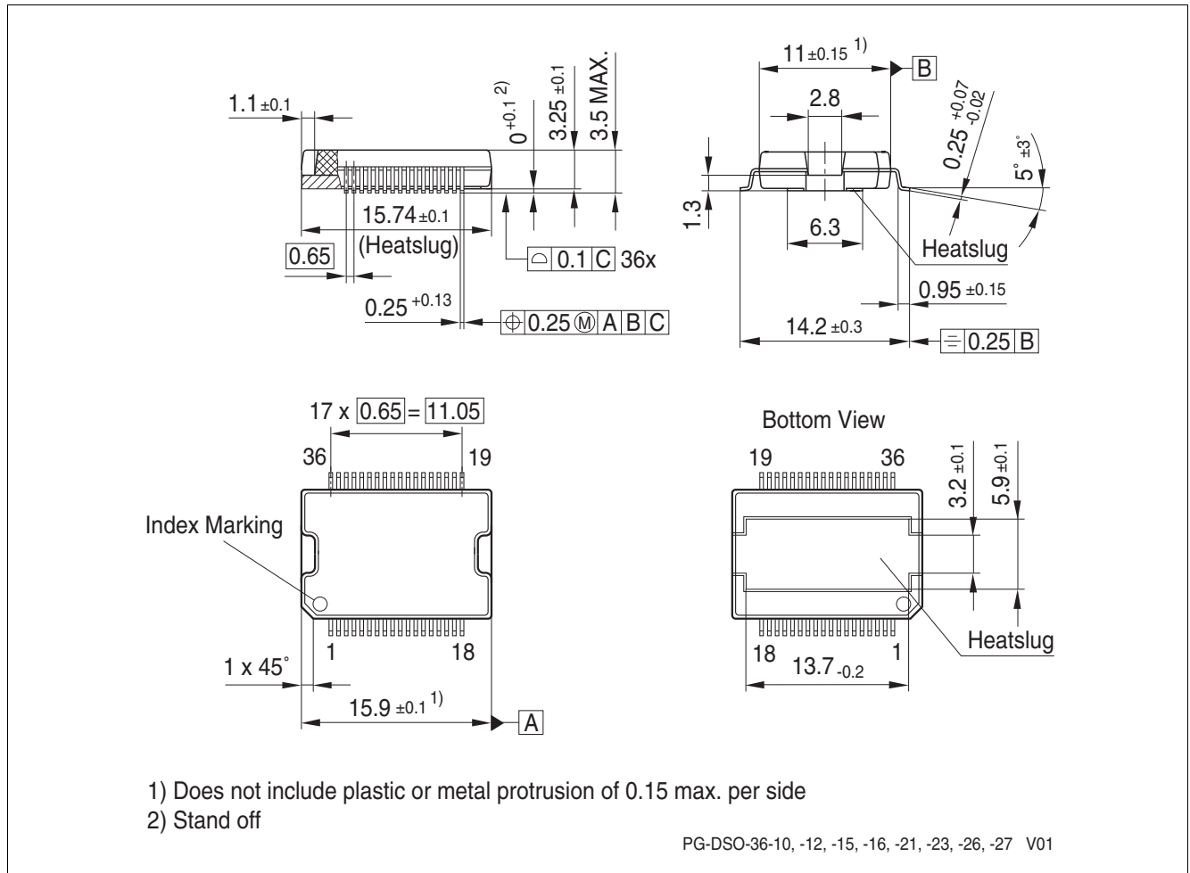
Figure 39 PG-DSO-36
