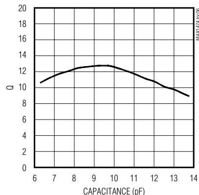
QUALITY FACTOR vs. CAPACITANCE
