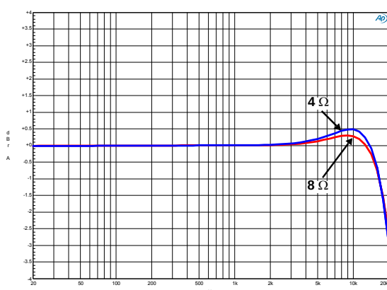
Figure 49. Frequency Response - FHD Mode
