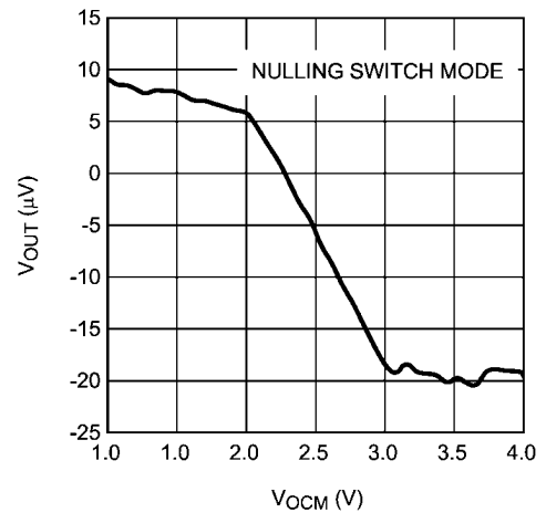
Vos vs. Input Common Mode Voltage
