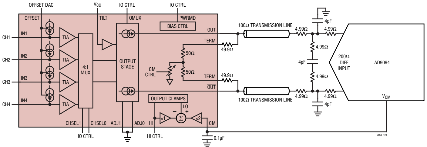
Figure 19. LTC6563 100Ω Transmission Line Circuit
