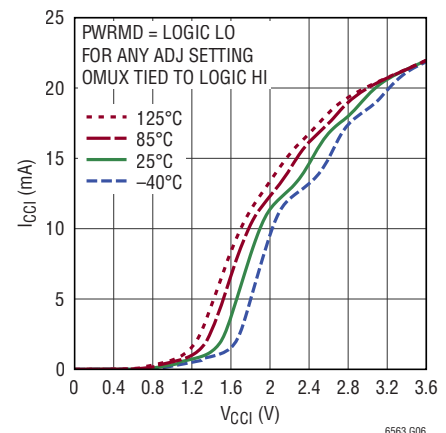
I_{\text{CCI}} vs V_{\text{CCI}} Over Temperature
