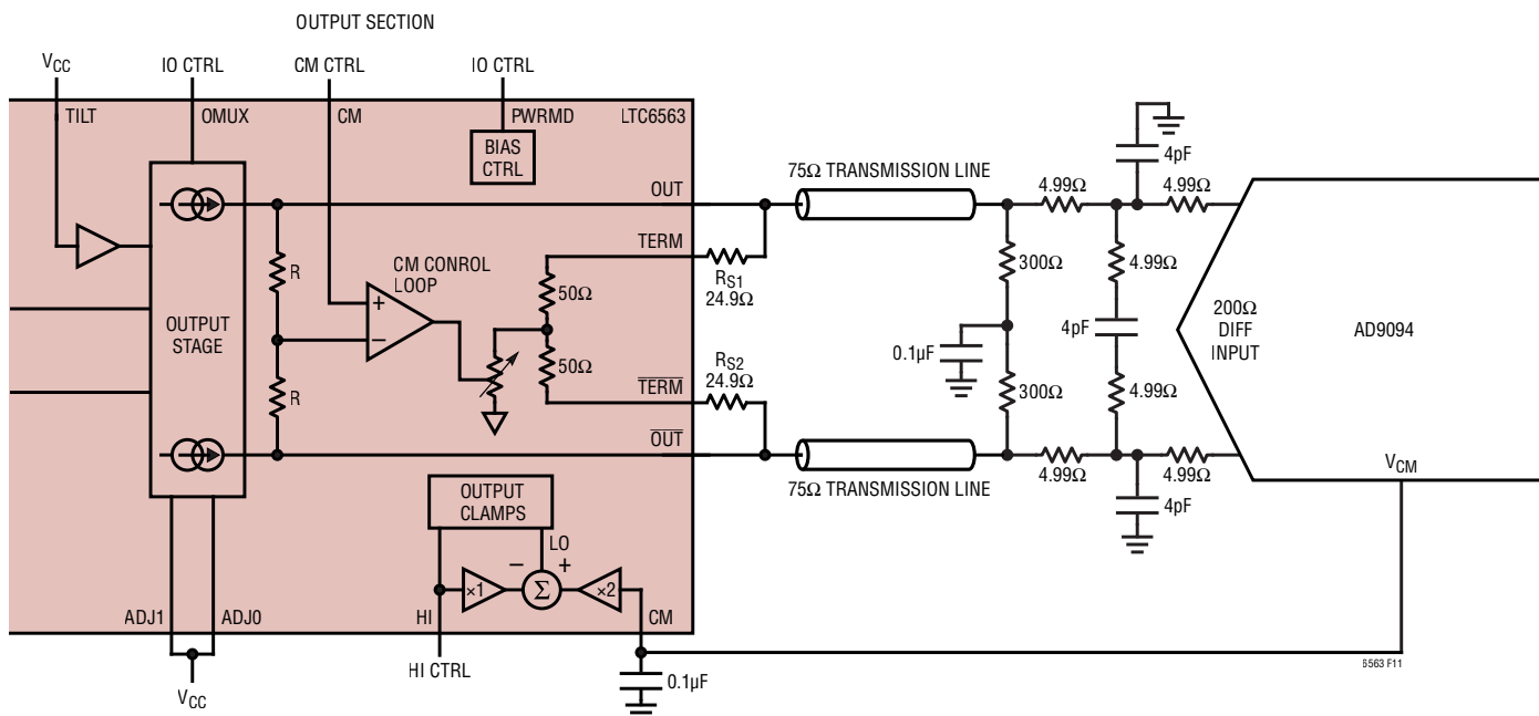
Figure 11. Increasing Diff Load Resistance and Matching to 75Ω
