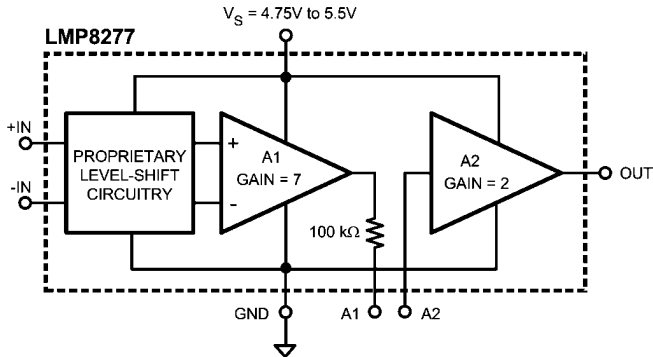
FIGURE 1. LMP8277
