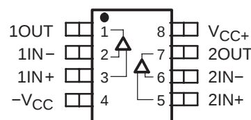
THS4052 D AND DGN† PACKAGES (TOP VIEW)
