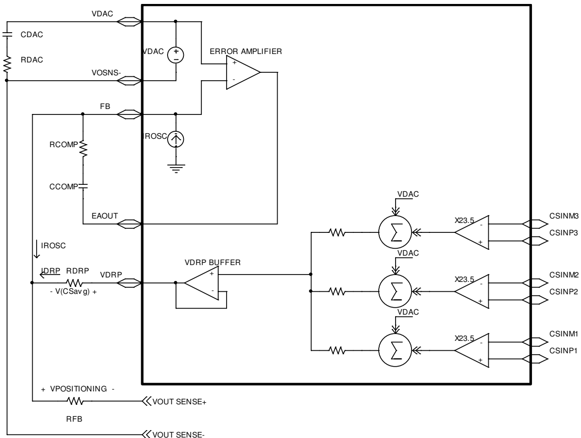
A resistor RFB between FB pin and the converter output is used to create output voltage offset VO_NLOFST which is the difference between VDAC voltage and output voltage at no load condition. An internal current source whose value is programmed by the same external resistor that programs the oscillator frequency, RROSC, pumps current IFB out of the FB pin.
