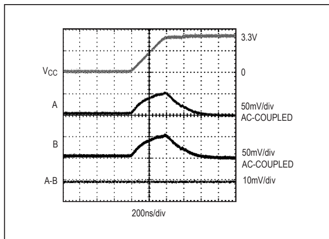
Figure 12. Differential Power-Up Glitch (10V/μs)
