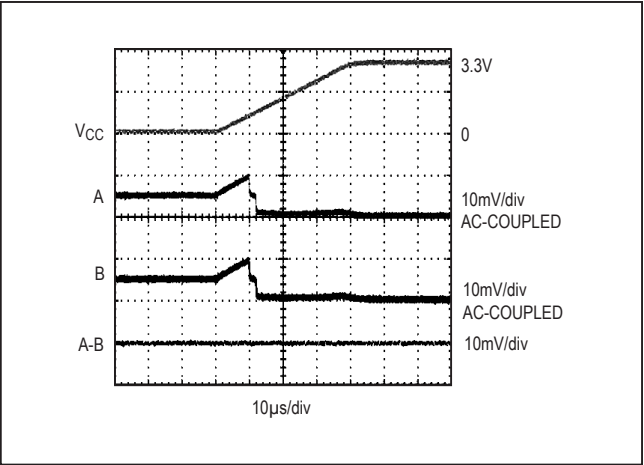
Figure 10. Differential Power-Up Glitch (0.1V/µs)
