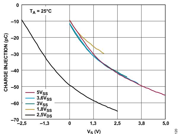
Figure 19. Charge Injection vs. V_S
