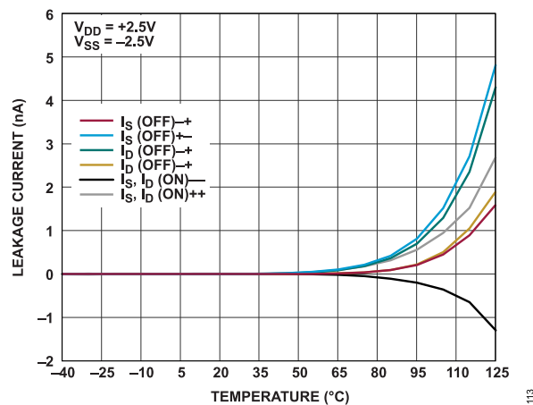
Figure 12. Leakage Current vs. Temperature, 2.5 V Dual Supply
