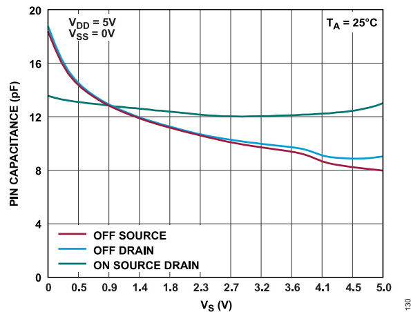
Figure 28. Pin Capacitance vs. V_S
