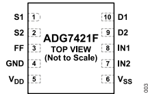
Figure 2. Pin Configuration
