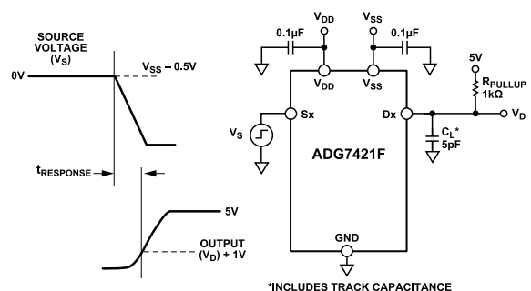
Figure 44. Negative Overvoltage Response Time, Single-Supply, t_{\text{RESPONSE}}
