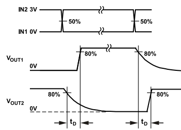
Figure 42. Break-Before-Make Time Delay, t_D
