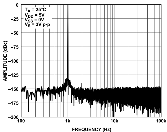
Figure 23. THD FFT
