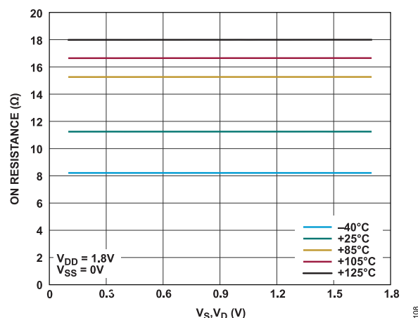
Figure 7. On Resistance as a Function of V_S , V_D for Different Temperatures, 1.8 V Single Supply
