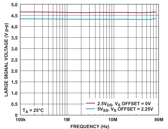
Figure 32. Large Voltage Signal Voltage vs. Frequency
