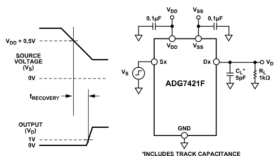
Figure 45. Overvoltage Recovery Time, t_{\text{RECOVERY}}
