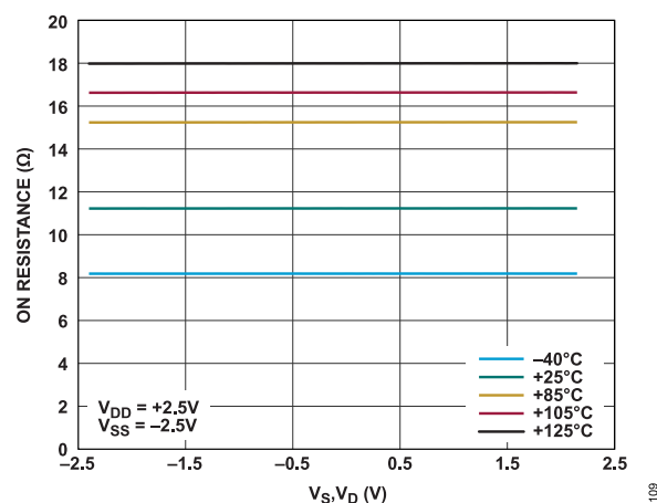
Figure 8. On Resistance as a Function of V_S , V_D for Different Temperatures, 2.5 V Dual Supply
