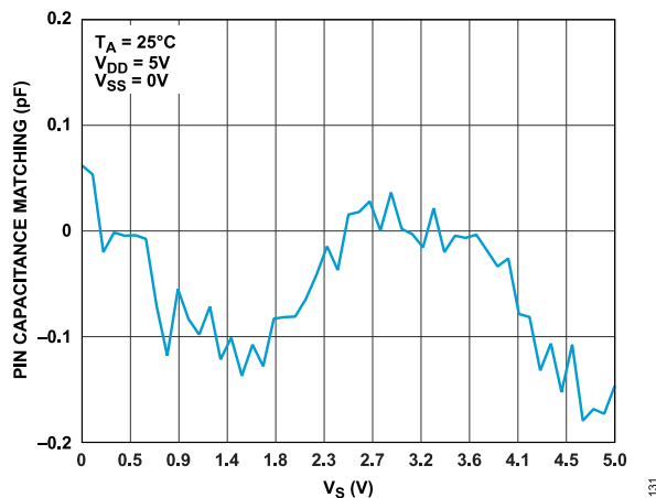
Figure 29. Pin Capacitance Matching vs. V_S
