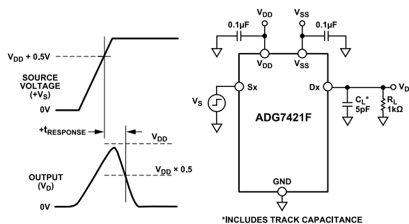
Figure 43. Overvoltage Response Time, t_{\text{RESPONSE}}
