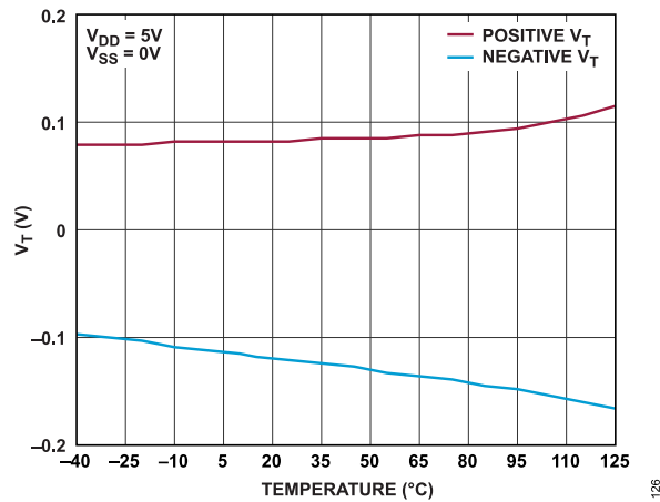
Figure 27. V_T vs. Temperature, 5 V Single Supply
