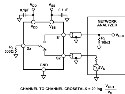
Figure 39. Channel to Channel Crosstalk
