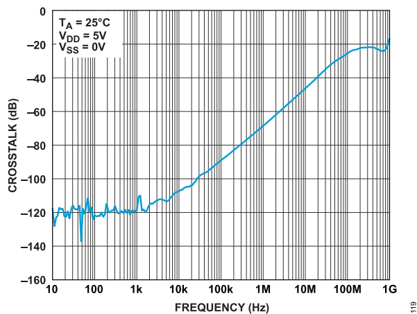
Figure 18. Crosstalk vs. Frequency, 5 V Single Supply
