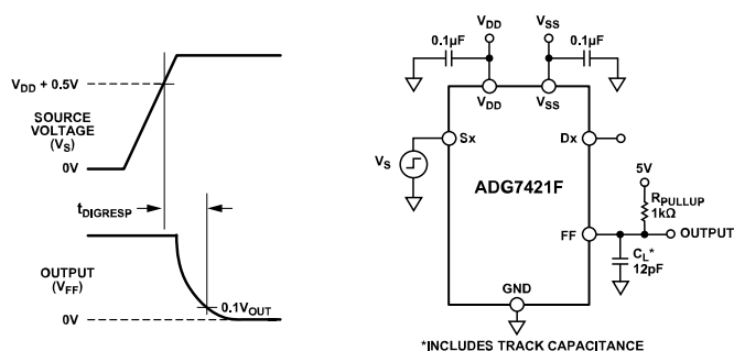
Figure 46. Interrupt Flag Response Time, t_{\text{DIGRESP}} ( V_{\text{FF}} is the Fault Flag Voltage)
