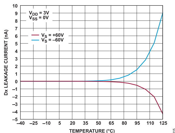
Figure 14. Dx Leakage Current vs. Temperature During Overvoltage, 3 V Single Supply
