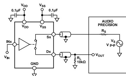
Figure 41. THD + N
