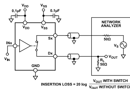
Figure 40. Bandwidth
