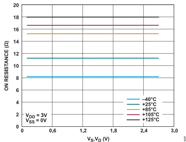
Figure 6. On Resistance as a Function of V_S , V_D for Different Temperatures, 3 V Single Supply
