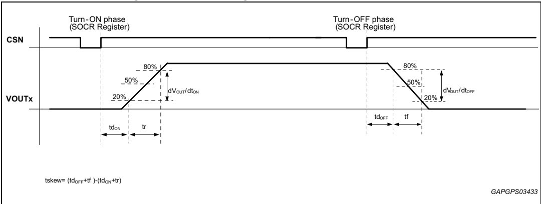
Figure 26. Switching characteristics
