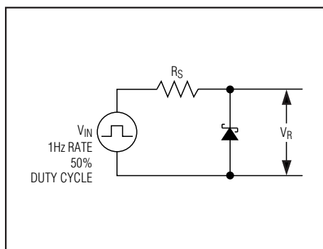
Figure 2. Startup Characteristics Test Circuit
