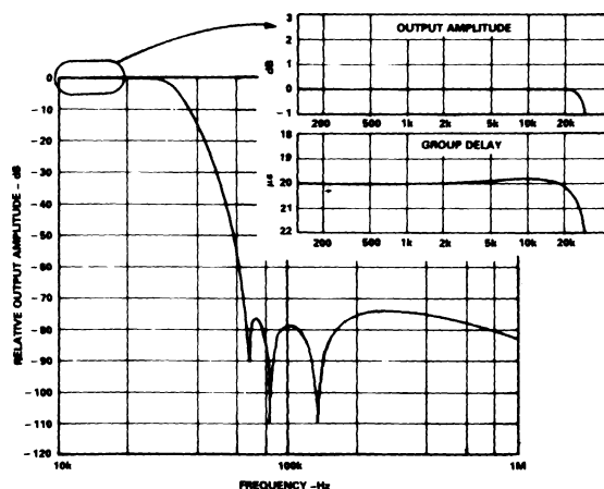
Figure 44. Relative Output Amplitude vs. Frequency of Antialiasing Filter
