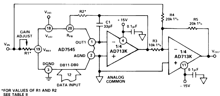
Figure 39. Bipolar Operation
