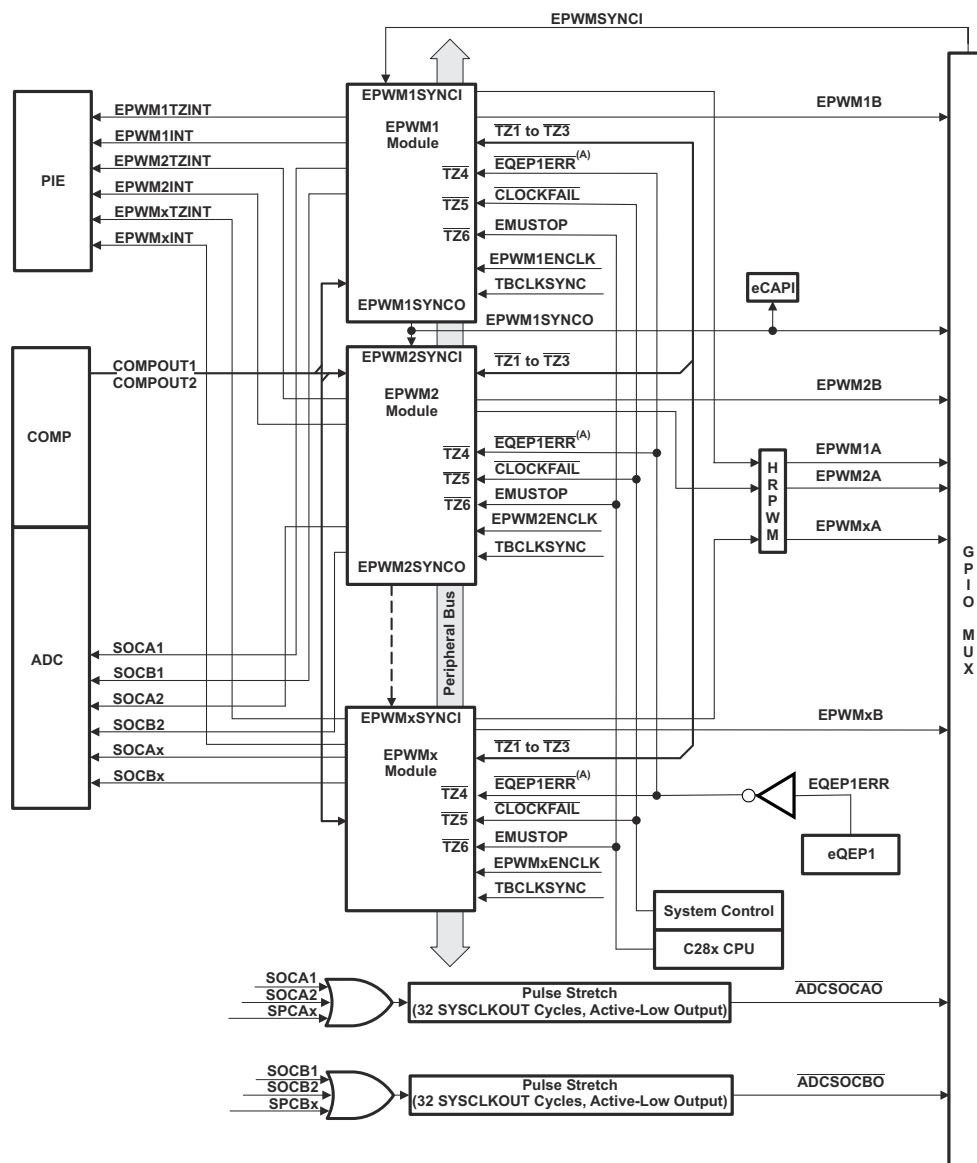
Figure 8-38. ePWM
