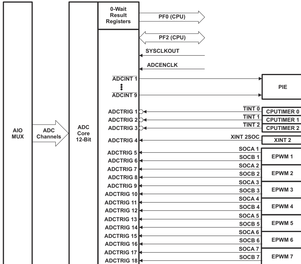
Figure 8-17. ADC Connections
