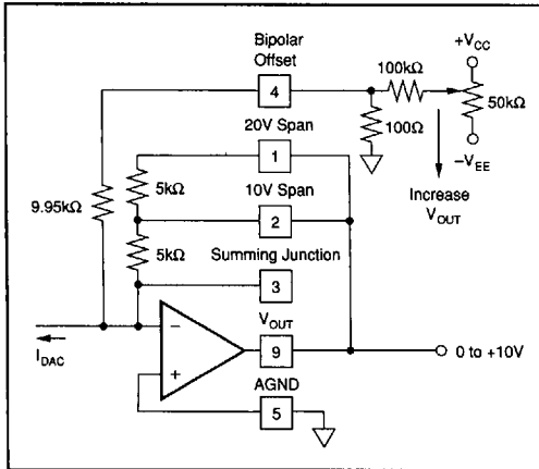
FIGURE 7. 0 to +10V Unipolar Voltage Output.
