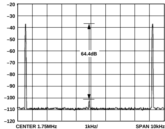
Figure 39. In-Band MTPR at 1.751 MHz
