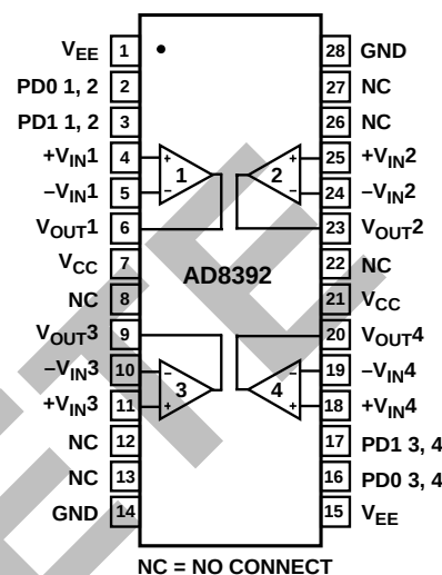
Figure 1. AD8392ARE, 28-Lead TSSOP/EP
