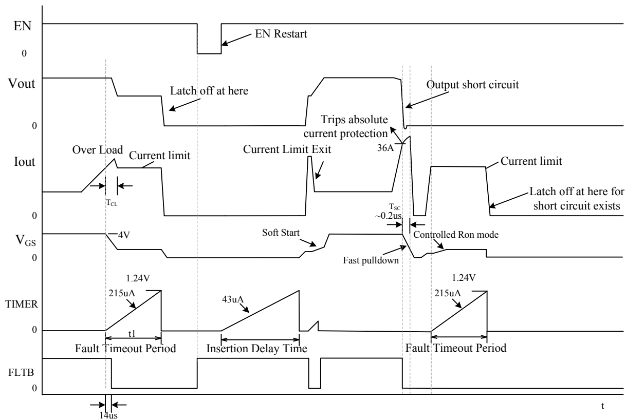
Figure 2: Over-Current Protection
