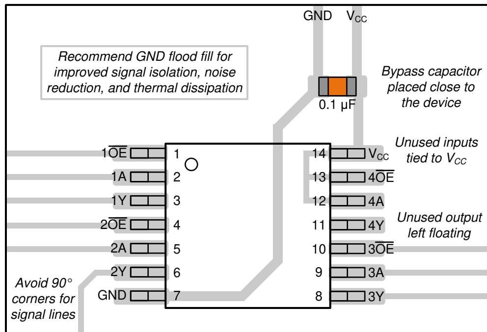
Figure 11-1. Example Layout for the SNx4AHCT125
