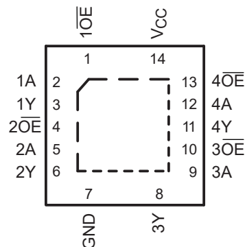
Figure 5-2. SN74AHCT125 RGY or BQA Package (Top View)
