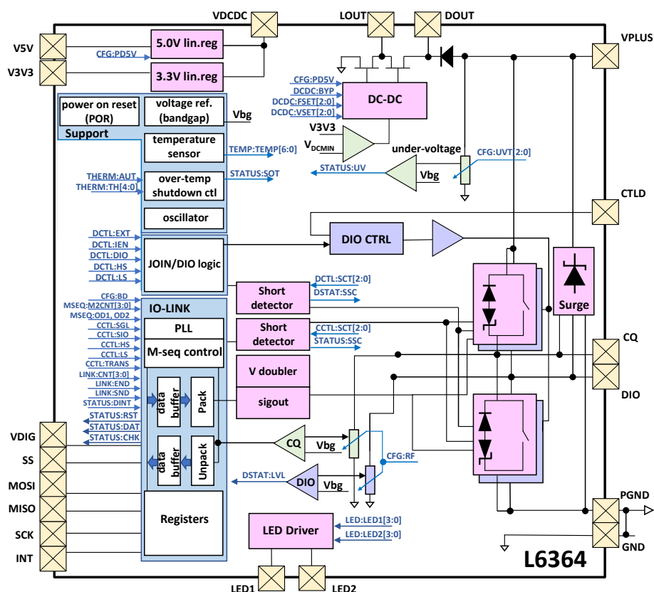
Figure 20. Detailed block diagram, showing register field connections
