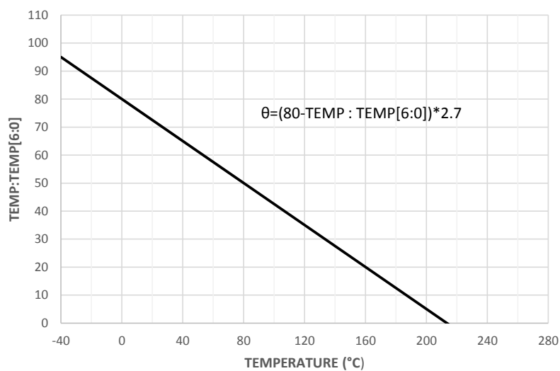
Figure 11. L6364 temperature measurement
