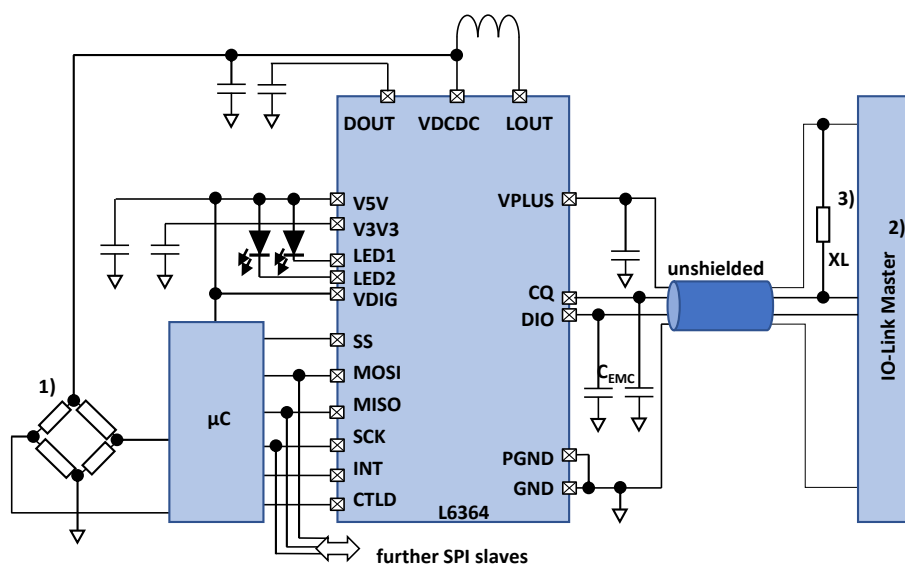
Figure 24. Application example: DC-DC enabled, CQ and DIO as independent line drivers, V_{\text{SENSOR}} > 5.0 \text{ V} , V_{\text{MCU}} = V_{\text{DIG}} = 5.0 \text{ V}
