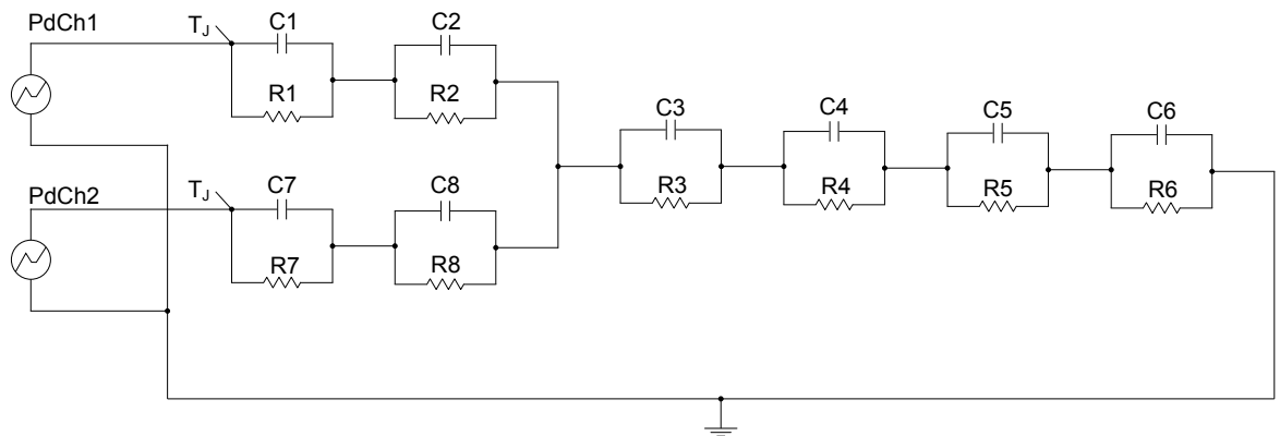
Figure 29. Thermal fitting model of a double channel HSD in PowerSSO-12
