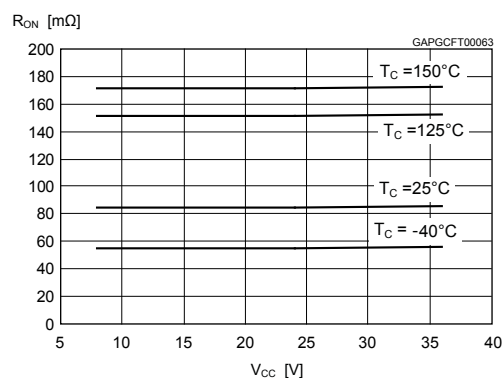
Figure 20. On-state resistance vs V_{CC}
