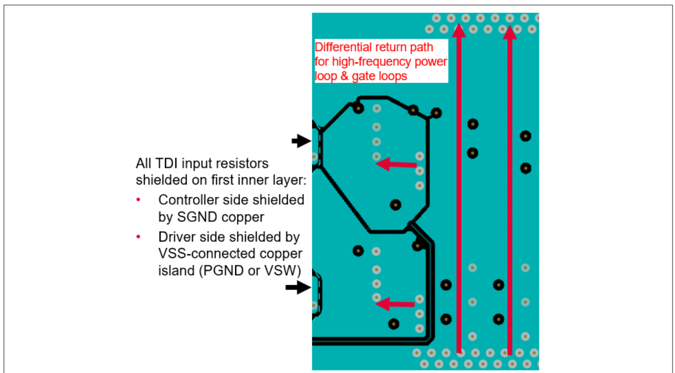
Figure 27 First inner layer of example half-bridge implementation, separated from top layer by 80~100 µm dielectric
