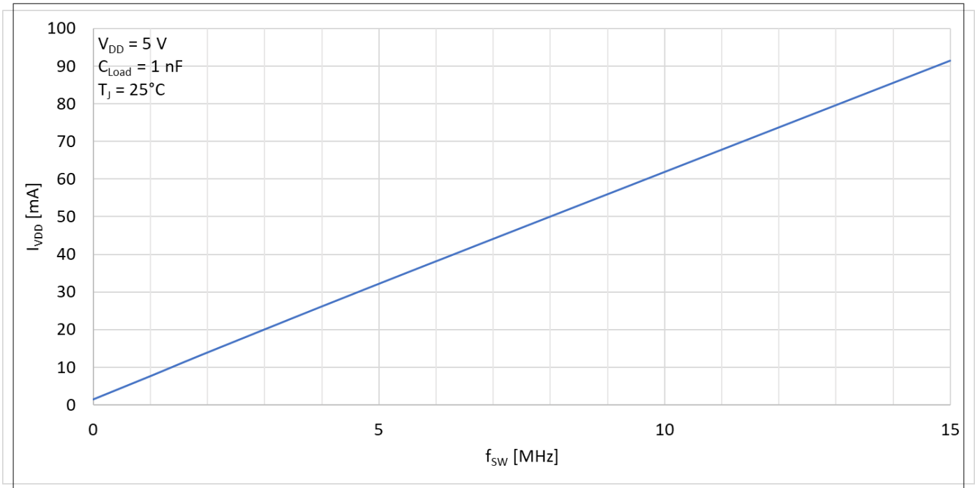
Figure 11 Operating current with load versus frequency
