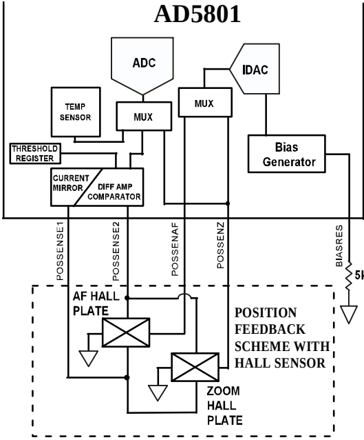
Figure 7. Lens Position Sensing using Hall Sensors.
