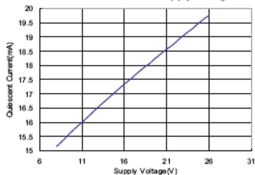
12. Quiescent Current vs Supply Voltage
