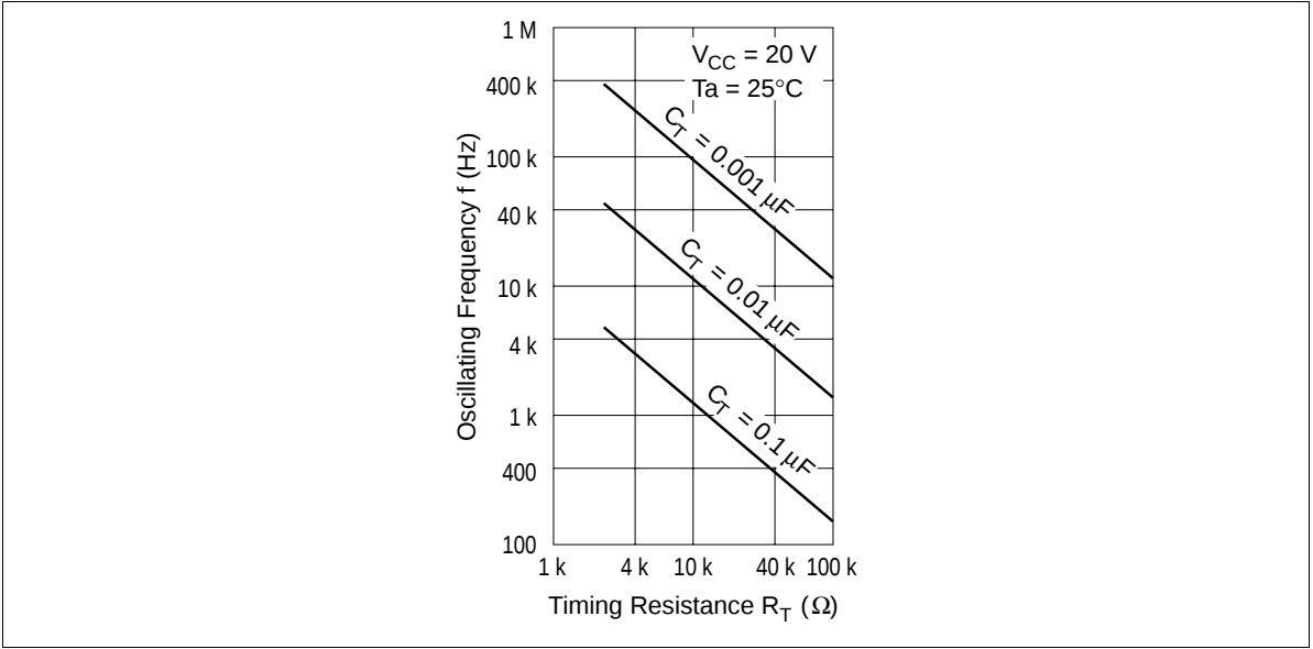
Figure 3 Oscillating Frequency vs Timing Resistance
