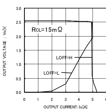
Fig.9 Load regulation
