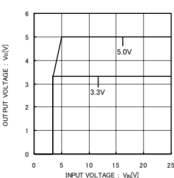
Fig.8 Line regulation
