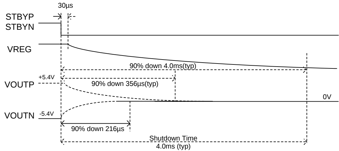
Figure 18. OFF Sequence Timing (STBYP=STBYN)
