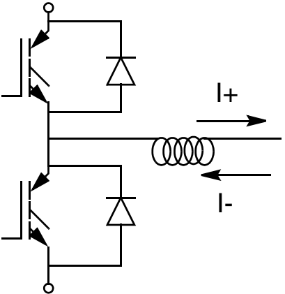
Figure 12-19. Current Convention
