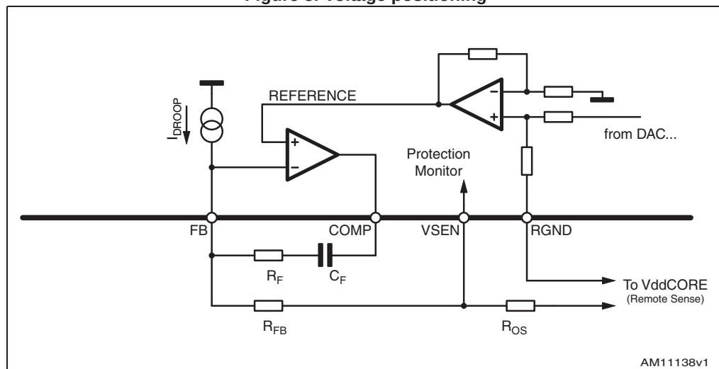
Figure 5. Voltage positioning
