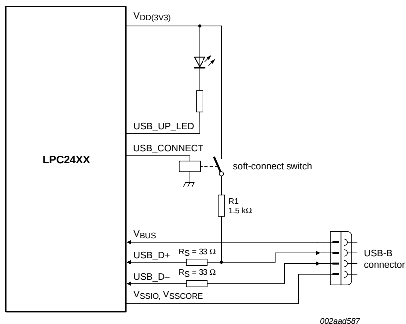
Fig 20. LPC2458 USB interface on a self-powered device
