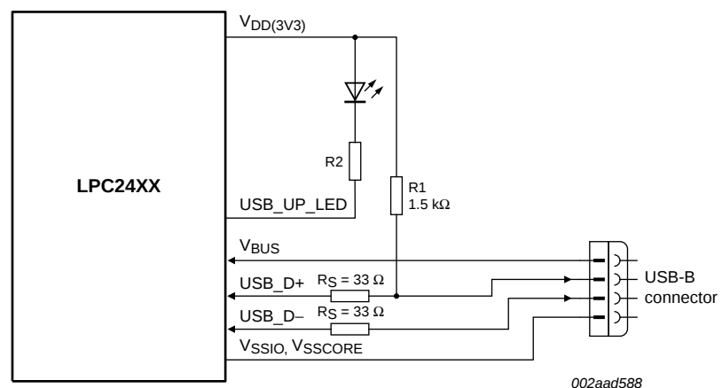
Fig 21. LPC2458 USB interface on a bus-powered device
