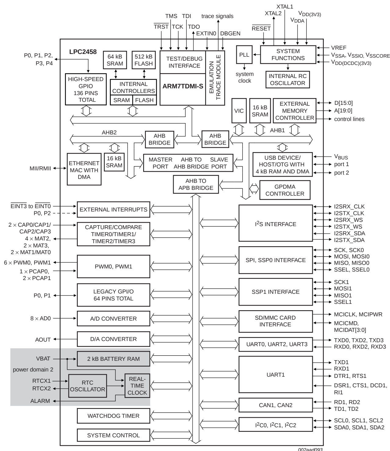
Fig 1. LPC2458 block diagram
