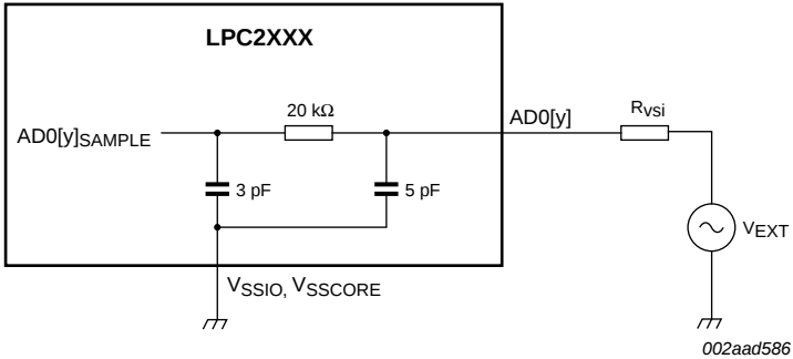
Fig 19. Suggested ADC interface - LPC2458 AD0[y] pin
