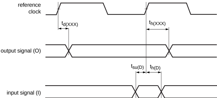
Fig 17. Signal timing
