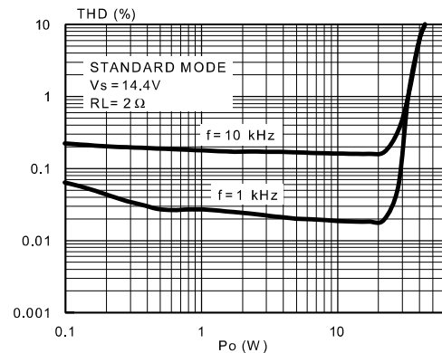
Figure 9. Distortion vs. output power (2 \Omega , STD)
