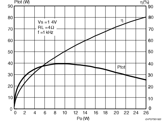
Figure 19. Total power dissipation and efficiency vs. output power (4 \Omega , STD, Sine)
