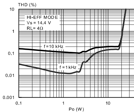
Figure 8. Distortion vs. output power (4 \Omega , HI-EFF)
