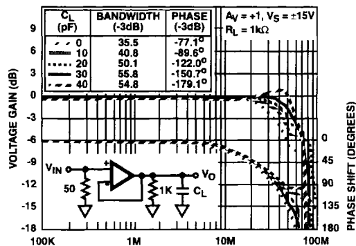
FIGURE 27. BANDWIDTH vs LOAD CAPACITANCE
