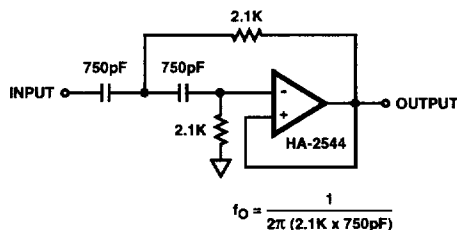
FIGURE 6. APPLICATION 3, 100\text{kHz} HIGH PASS 2-POLE BUTTERWORTH FILTER
