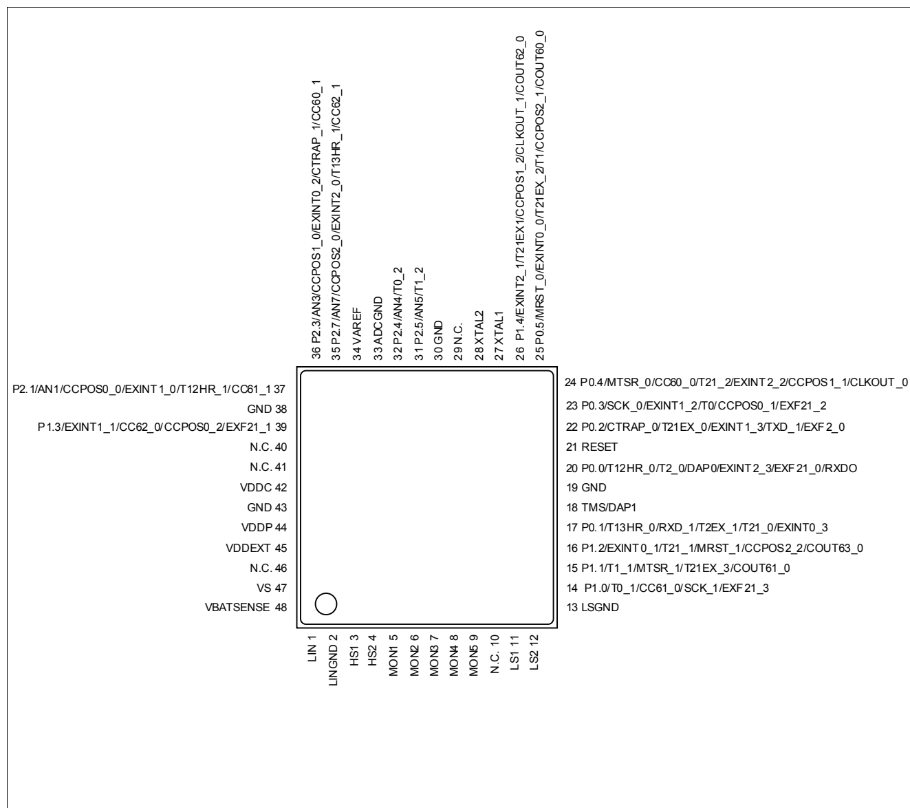
Figure 1 TLE9832-2 pin configuration, VQFN-48-22 and VQFN-48-29 packages (top view)
