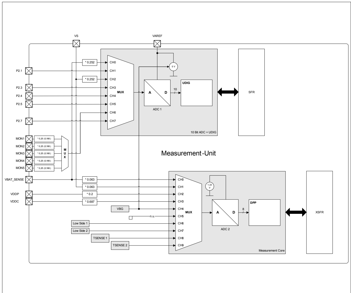
Figure 25 TLE9832-2 Measurement Unit-Overview
