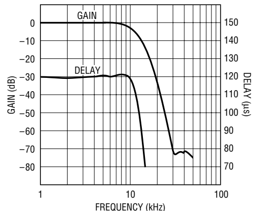
Frequency Response
