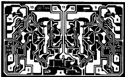
DIE SIZE 0.097 \times 0.063 inch, 6111 sq. mils ( 2.464 \times 1.600 mm, 3.94 sq. mm)
