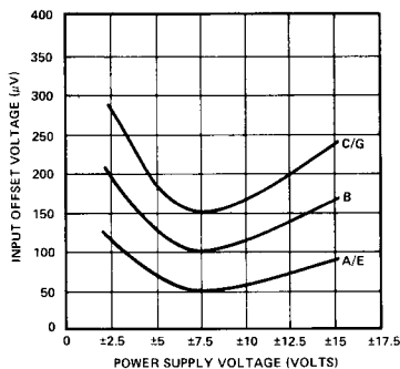
INPUT OFFSET VOLTAGE vs SUPPLY VOLTAGE
