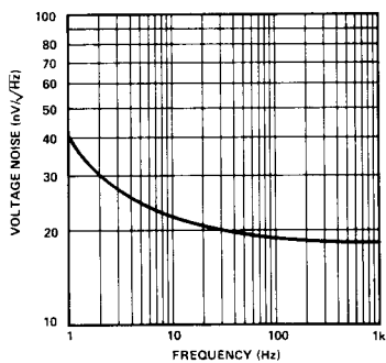
VOLTAGE NOISE DENSITY ( e_n ) vs FREQUENCY
