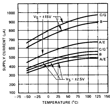
SUPPLY CURRENT vs TEMPERATURE AT V_S = \pm 15\text{V} AND \pm 2.5\text{V}
