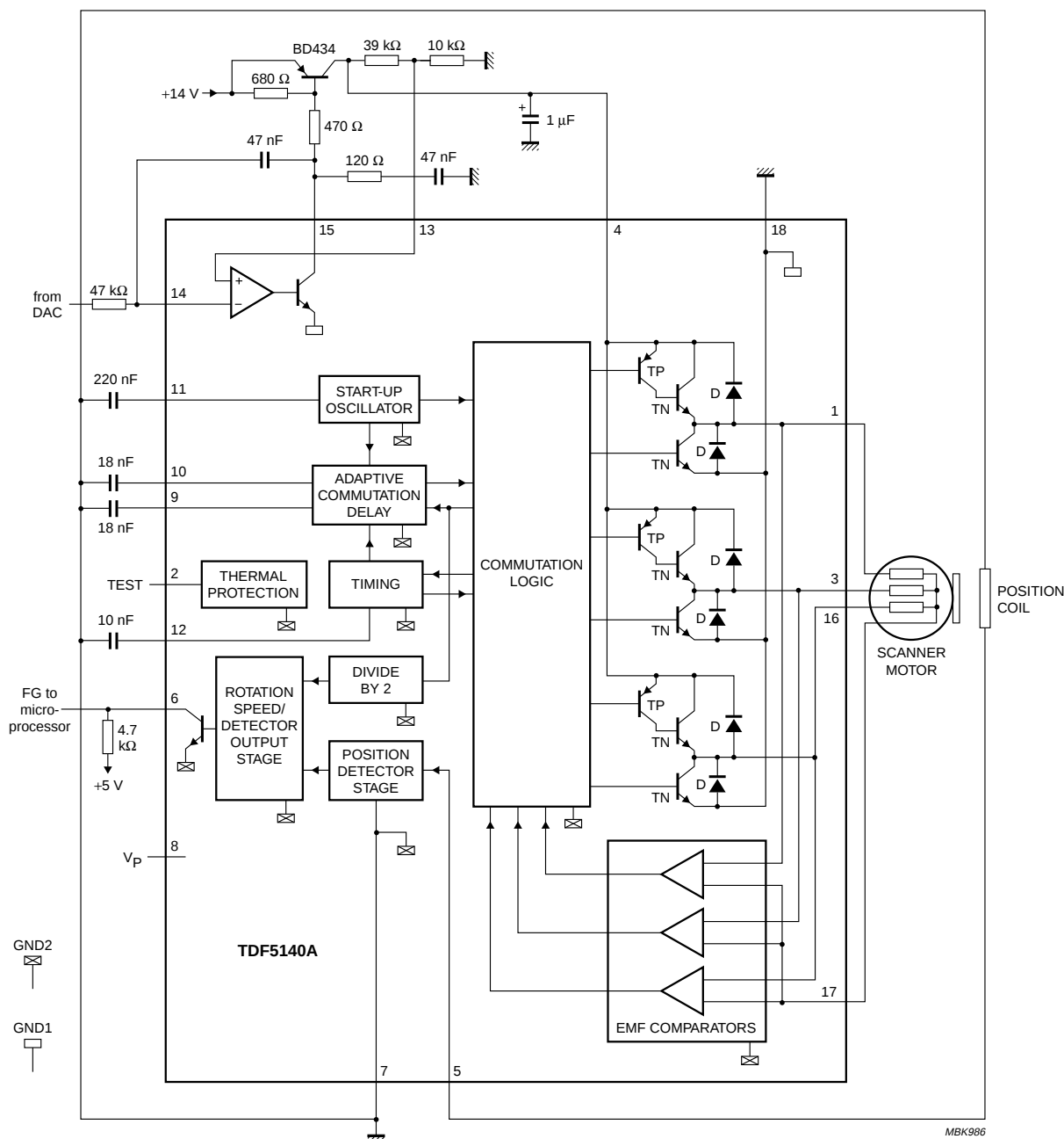
Fig.5 Typical application of the TDF5140A as a scanner driver, with use of OTA.
